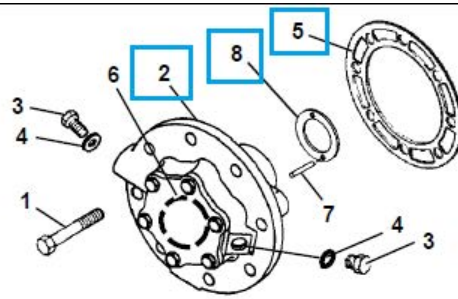
UNIVERSAL PUMP
