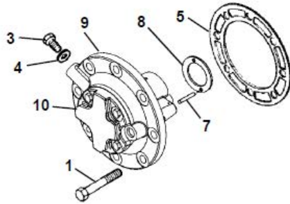
LOW PROFILE PUMP (NLO)
